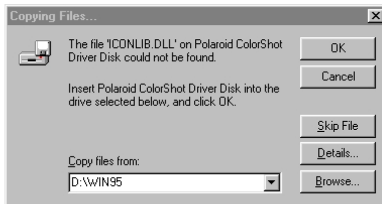
Windows 95
